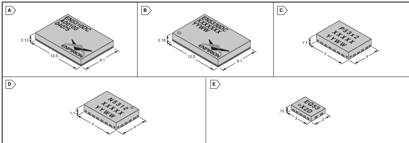
DIMENSIONS (mm)
